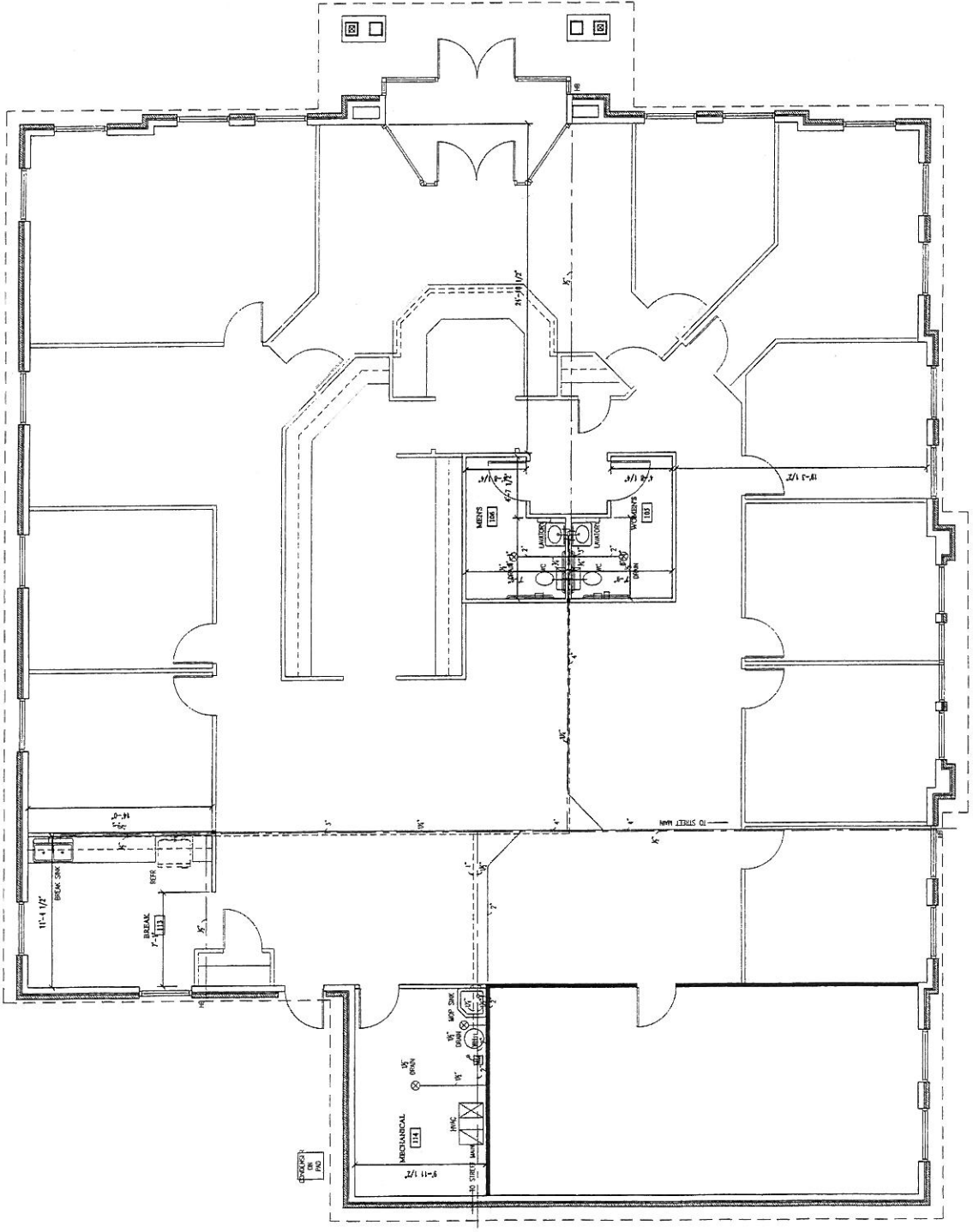
SUPPLY & SANITARY PLUMBING PLAN SCALE: 1/4" = 1'-0"
